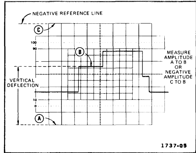
Fig. 17. Instantaneous voltage measurement.
