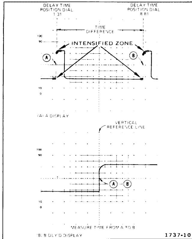
Fig. 27. Time difference between repetitive pulses.
