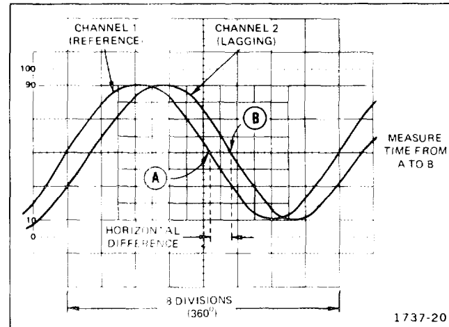
Fig. 23. Phase difference.
