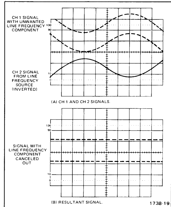
Fig. 19. Common-mode rejection.
