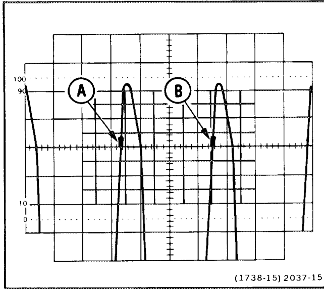
Fig. 15. DM44 timing check.
