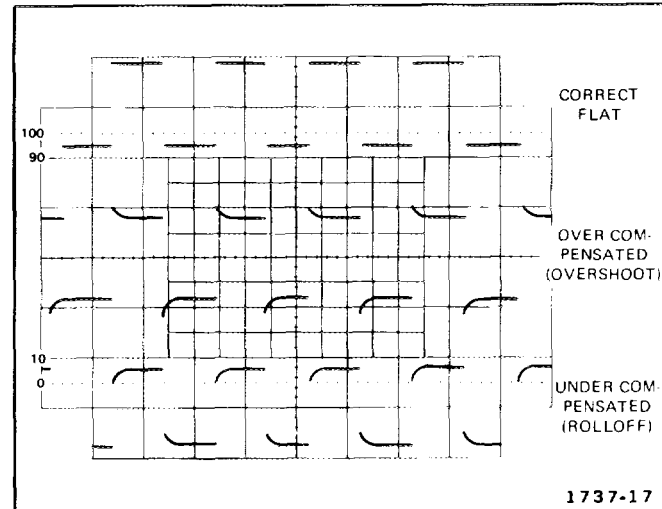
Fig. 13. Probe compensation.
