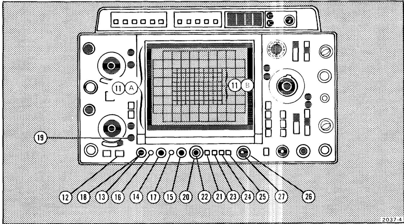
Fig. 3. Display and storage controls, connectors, and indicators.
