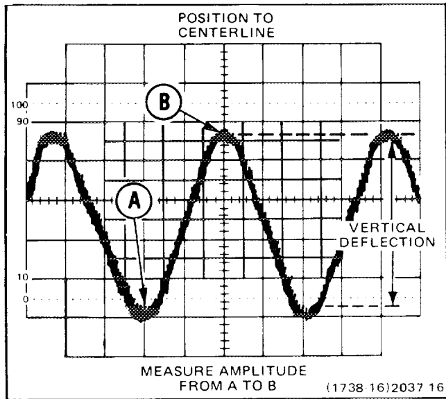
Fig. 16. Peak-to-peak voltage of a waveform.
