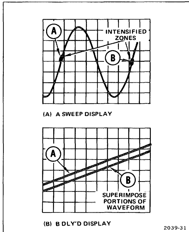
Fig. 32. Time duration and frequency measurements.
