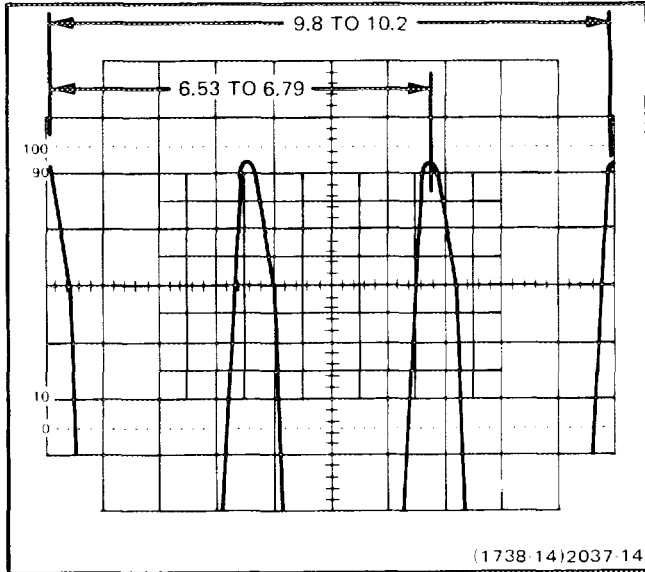
Fig. 14. Basic 466/464 timing check.
