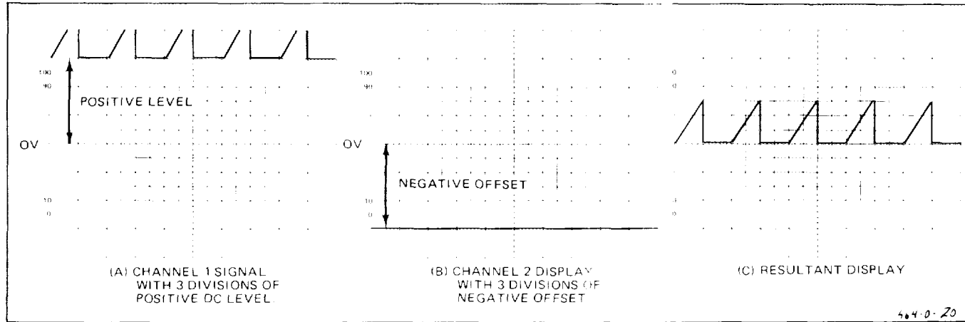
Fig. 18. Algebraic addition.
