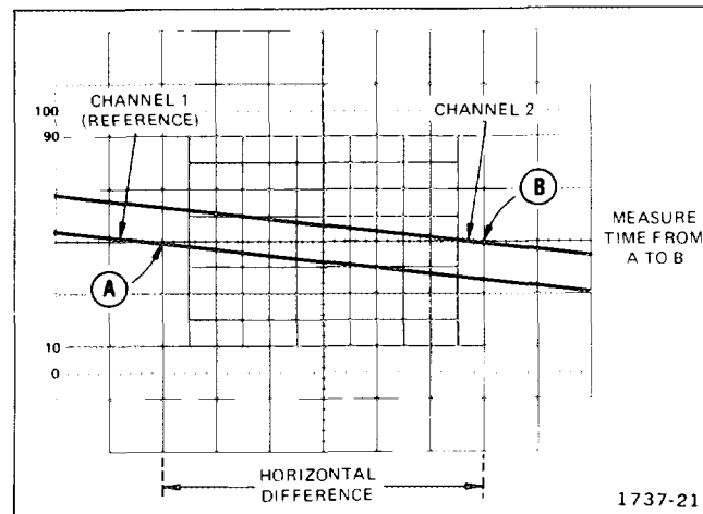
Fig. 24. High-resolution phase difference.
