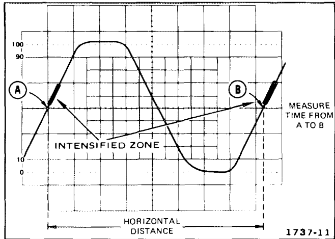
Fig. 28. Time duration.
