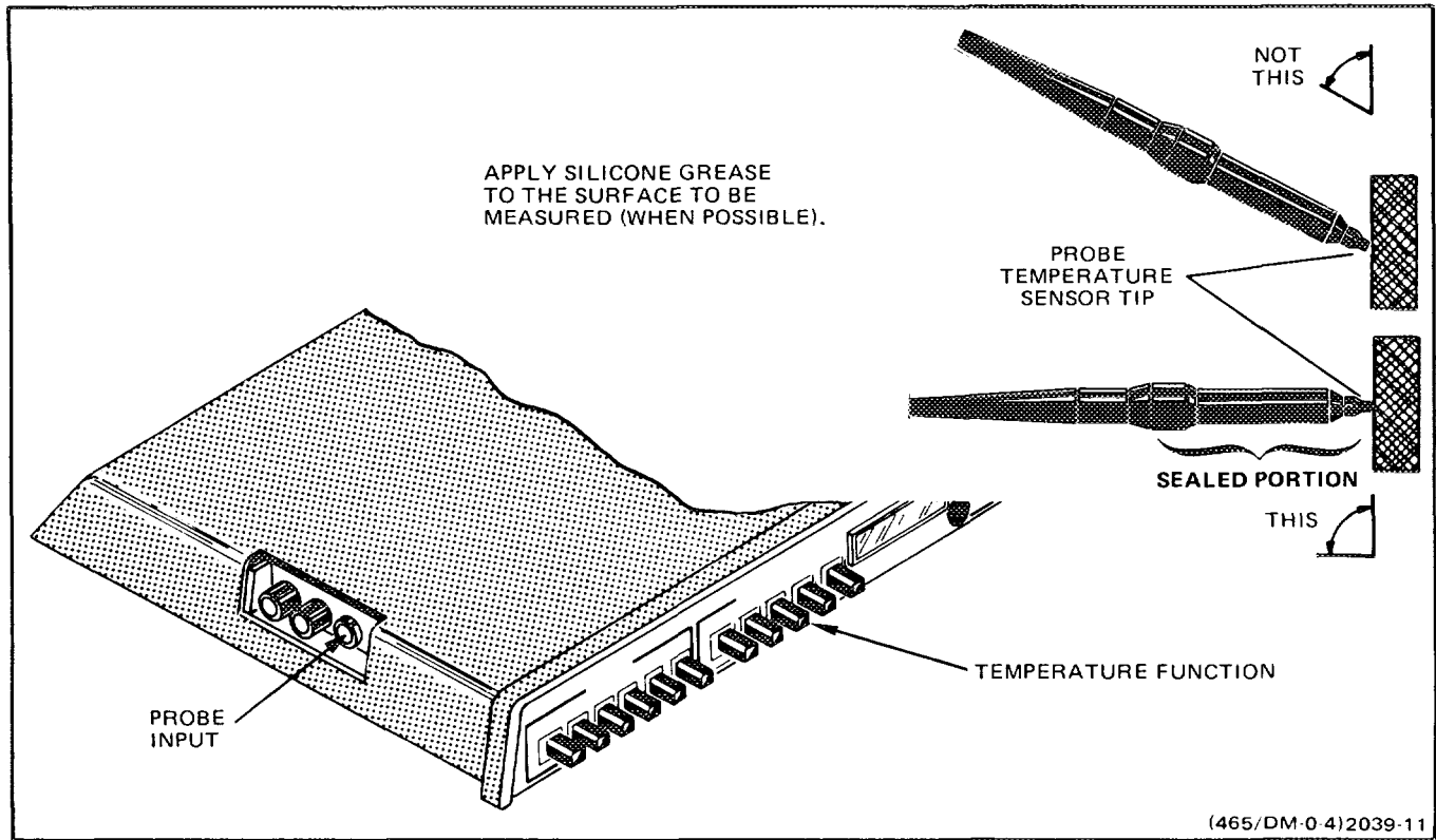
Fig. 12. Temperature.
