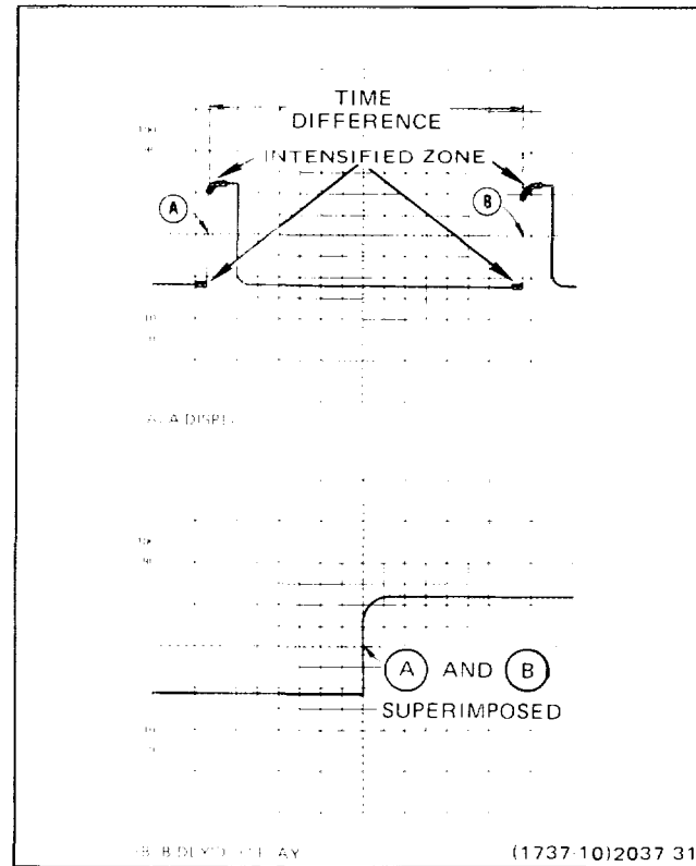
Fig. 31 Time difference between repetitive pulses.
